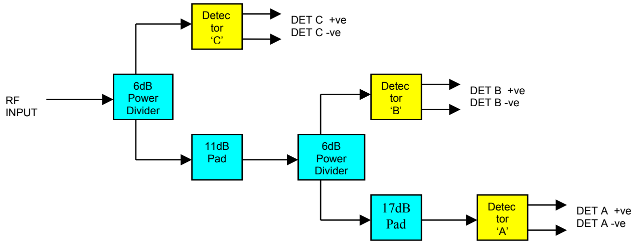
Fig 3: The MA2481B Universal Sensor
