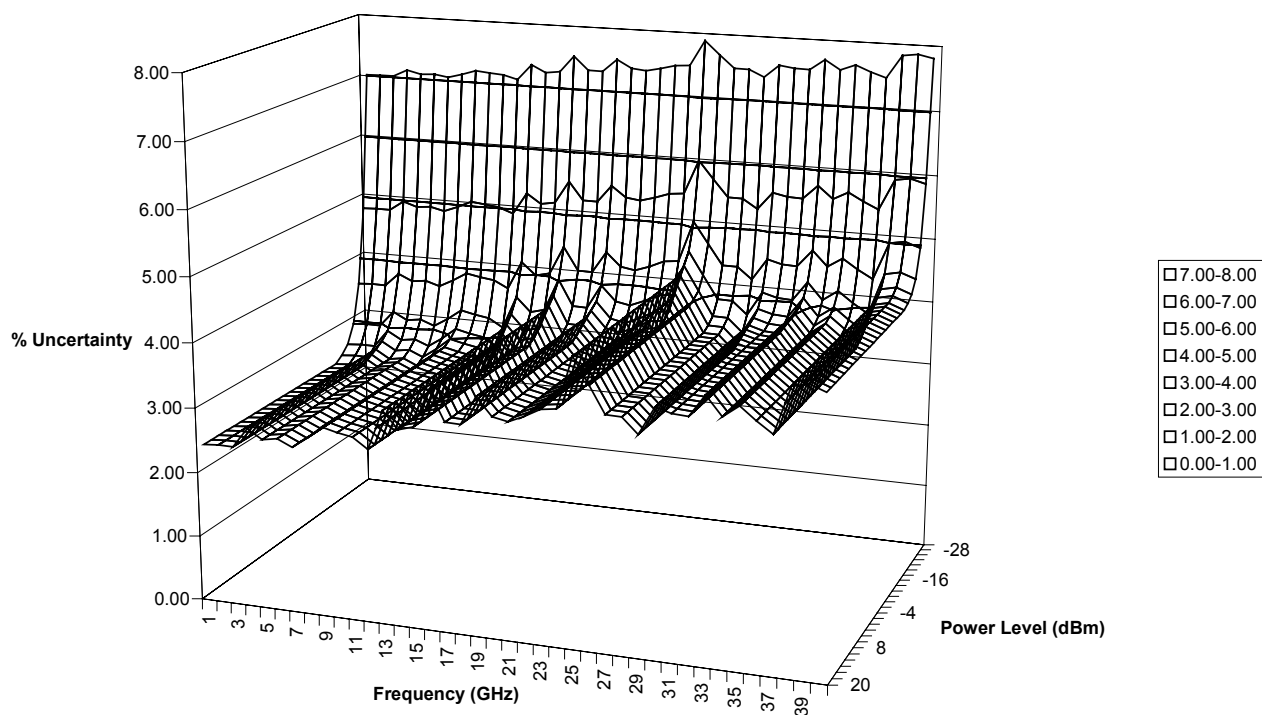
Thermal Sensor: RSS Uncertainties with 1.2 VSWR Source
