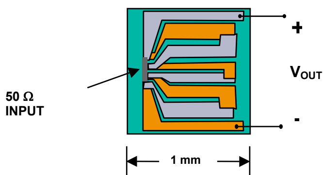
Figure 1: Thermopile Sensor THERMAL SENSOR
